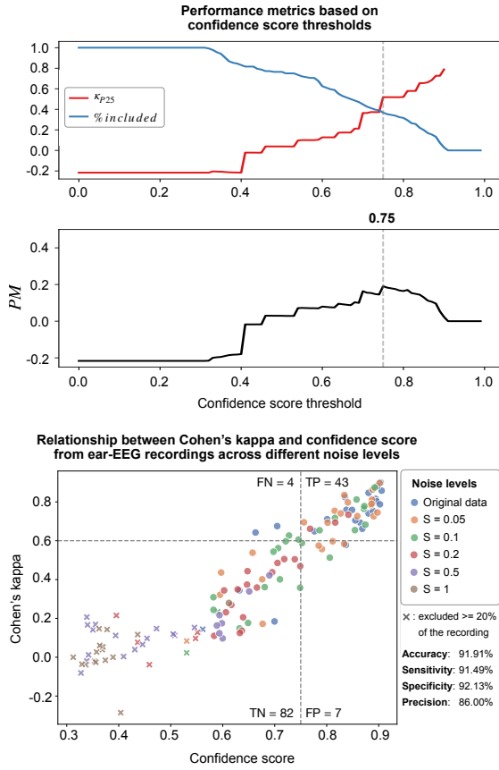
Fig. 3. Visualization of performance metrics across confidence score thresholds (upper) and the scatter plot, illustrating the correlation between \kappa values and confidence scores for both actual and simulated data (lower). The gray dashed line in the upper panel indicates the threshold determined for the optimal performance metric, which is also applied to the lower figure.
